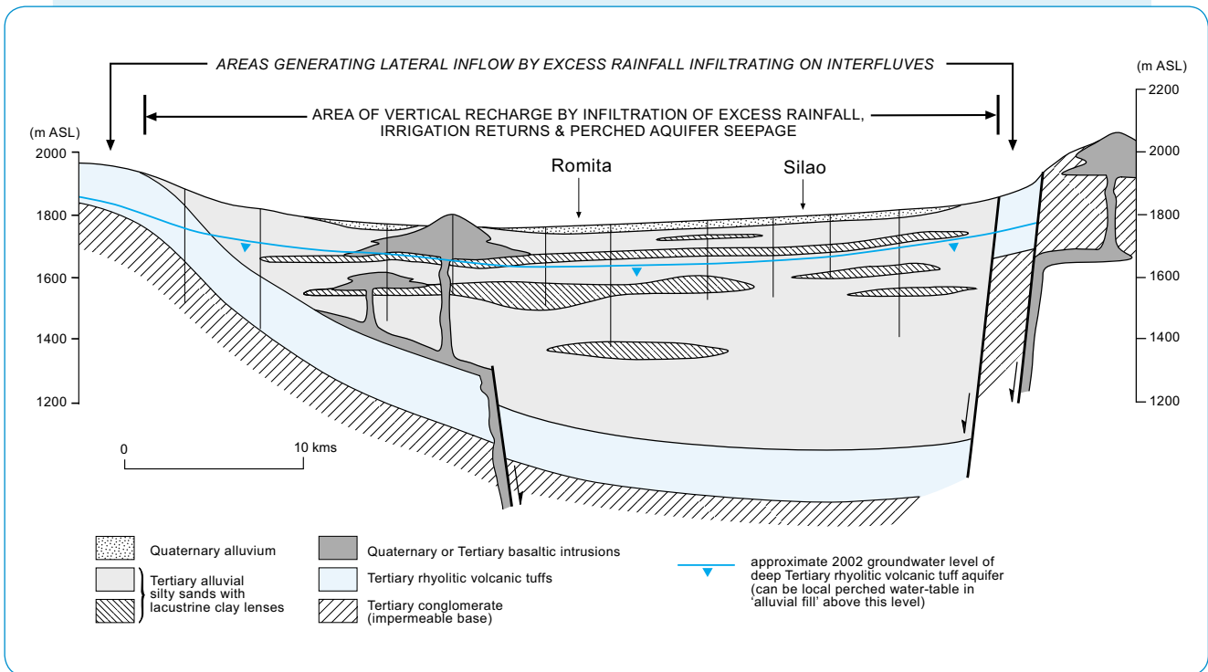
Figure 2: Schematic hydrogeological cross-section of the Silao-Romita aquifer system
