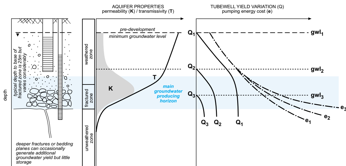
Figure 2: Hydraulic characteristics of the weathered Deccan Traps Basalt Aquifer and their effect on tube well yield-drawdown-energy consumption with rapidly deteriorating performance under falling water-table
