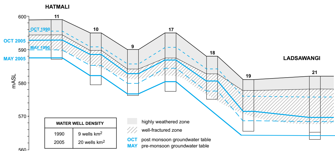
Figure 8: Variation of groundwater table levels in the main perennially-saturated aquifer of the Aurangabad MRWSSP pilot area during 1990-20
