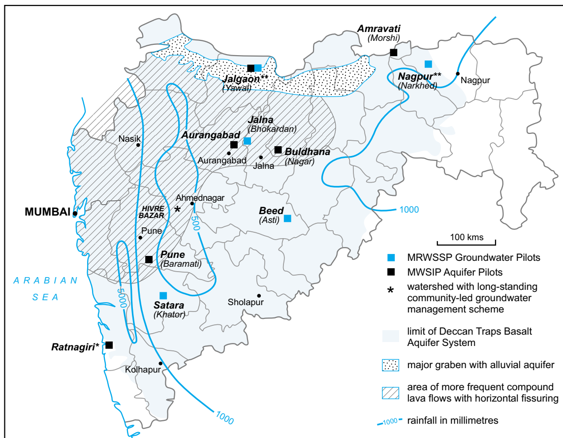
Figure 1: Hydrogeological map of Maharashtra State showing the extension of Deccan Traps Basalt and the location of MRWSSP & MWSIP Pilot Projects
