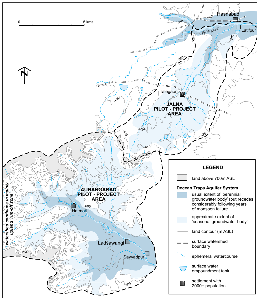
Figure 7: Hydrogeological sketch map of the Aurangabad MRWSSP & Jalna MWSIP pilot project areas to illustrate the occurrence of perennially-saturated groundwater bodies
