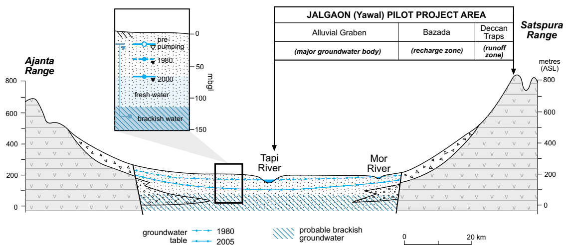
Figure 10: Generalised hydrogeological structure of the Tapi Gurnia Graben alluvial aquifer system showing the location of the Jalgaon District Pilot Project
