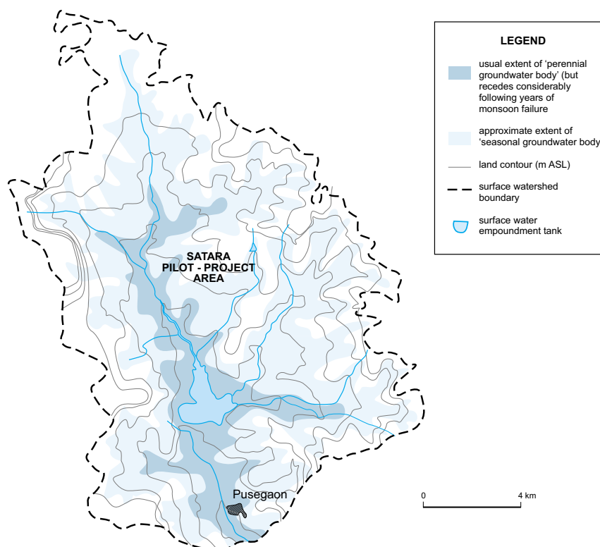
Figure 9: Hydrogeological sketch map of the Satara District MWSIP pilot project area to illustrate the occurrence of perennially-saturated groundwater bodies
