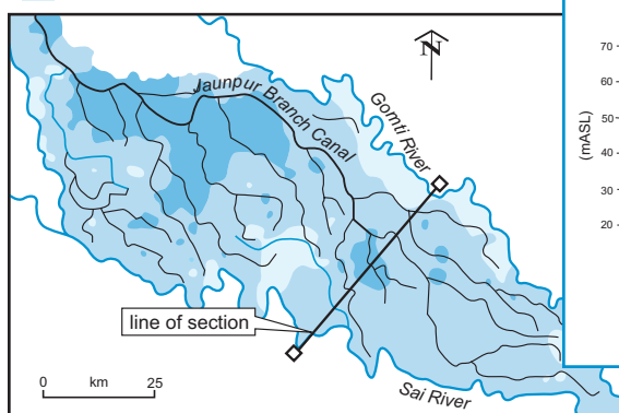
water-table depth (m bgl) in September 2005
